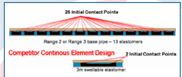
DynaFORM™ uses the unique SWELLFIX multi-element design, providing multiple initial contact points – the better the initial contact, the better the packer seals
